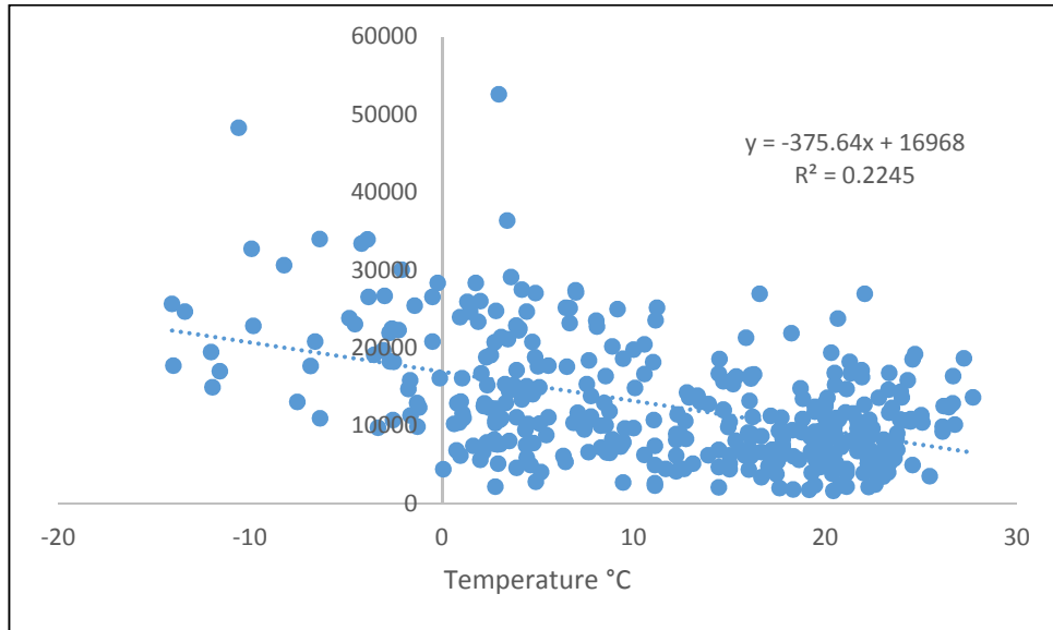
Figure 5: Effect of Temperature on Particle Count at Pembroke Site
