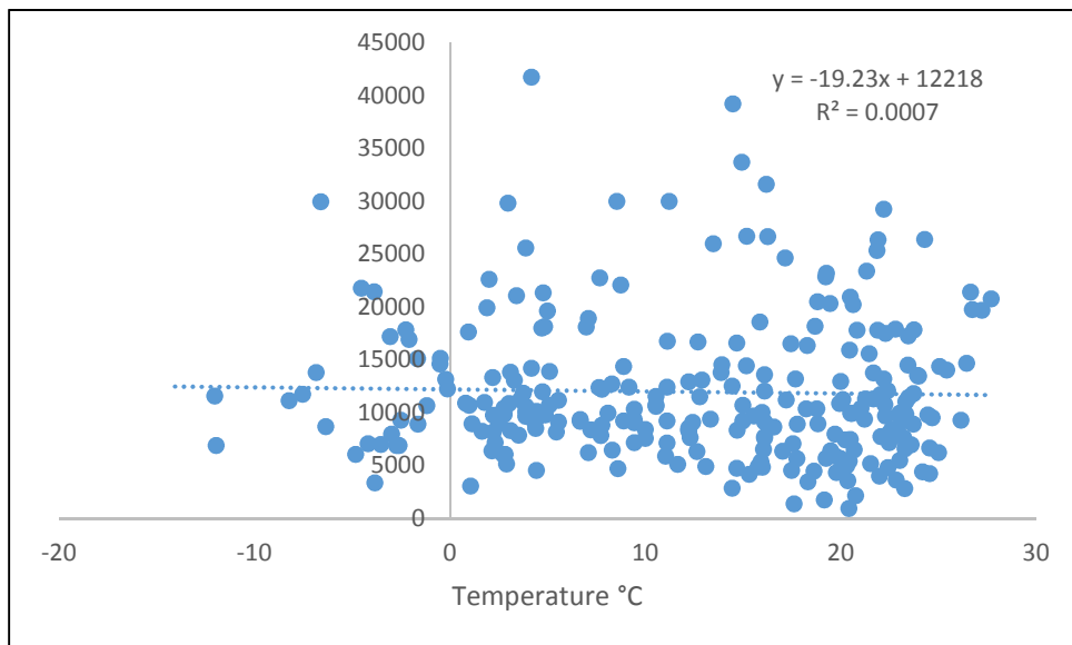
Figure 6: Effect of Temperature on Particle Count at Lydick Site
