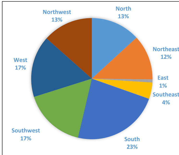
Figure 3: Percentage of Days with Each Prevailing Wind Direction
