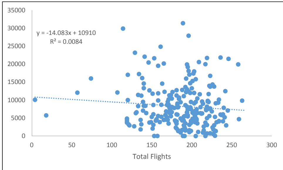
Figure 10: Effect of the Number of Flights on Particle Count at Field View Site
