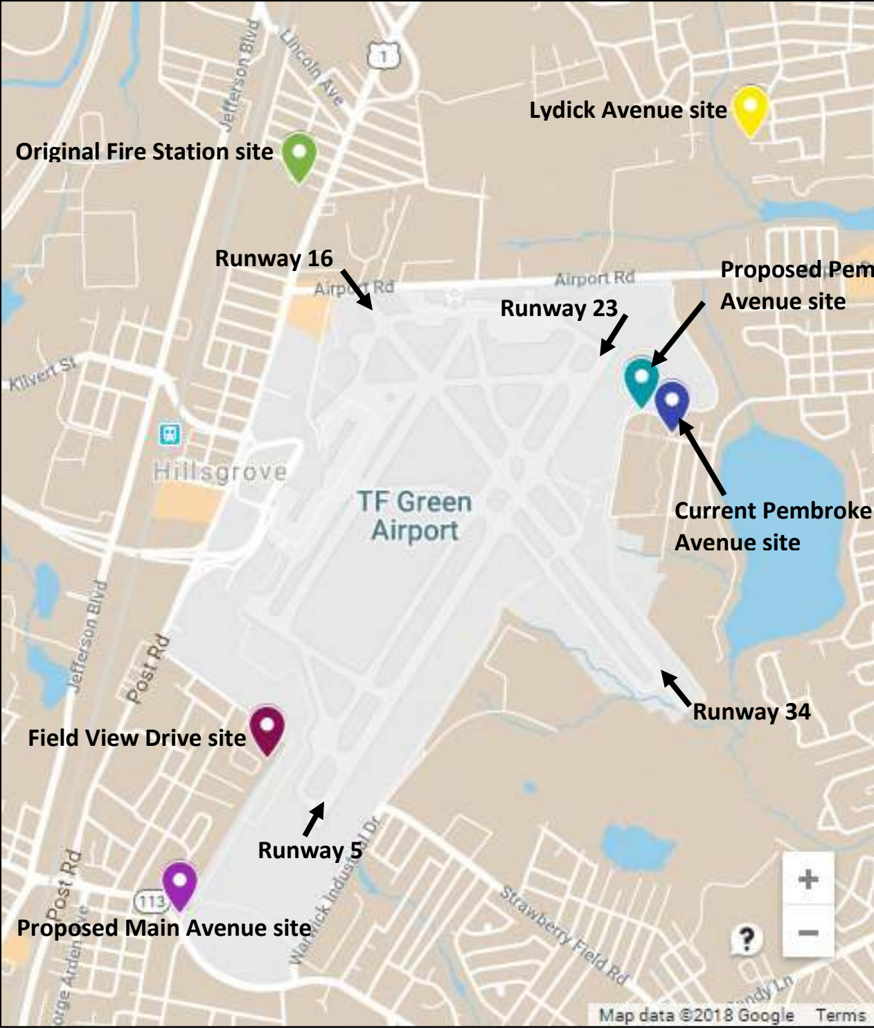
Figure 1: Current and Proposed Locations of RIAC Monitoring Sites and Locations of Runways
