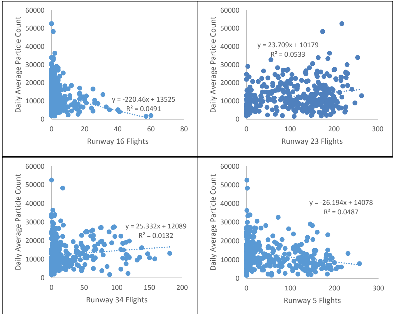
Figure 11: Effect of the Number of Flights, Using Each Runway, On Particle Count at the Pembroke Site
